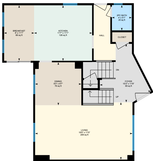
MAIN FLOOR
